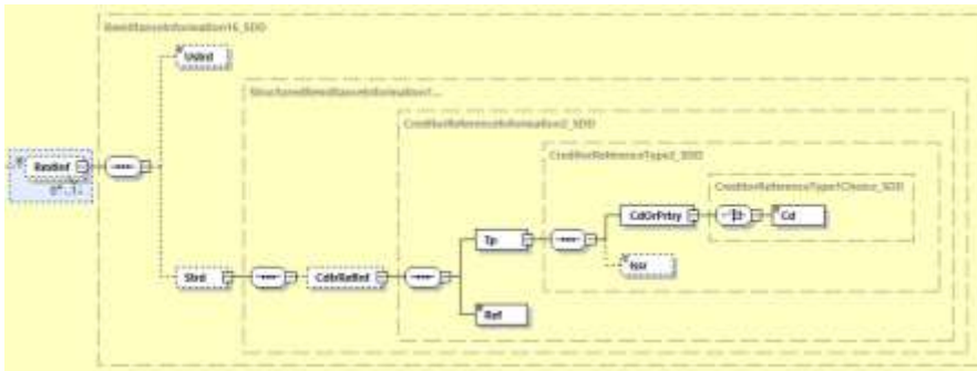
Abbildung 26: pain.008.001.08, Remittance Information
