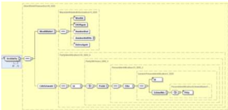
Abbildung 24: pain.008.001.08, Direct Debit Transaction
