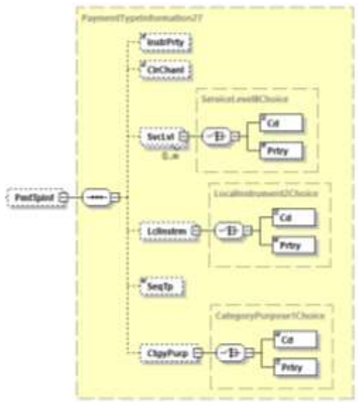
Abbildung 36: pain.002.001.10, Payment Type Information
