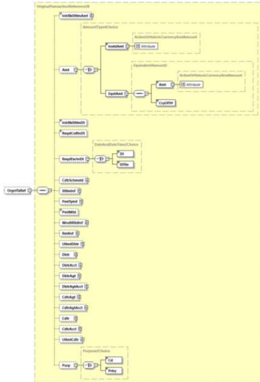
Abbildung 71: p:ain.002.001.10 , Original Transaction Reference
