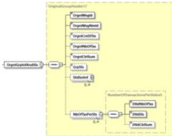
Abbildung 33: pain.002.001.10, Original Group Information and Status
