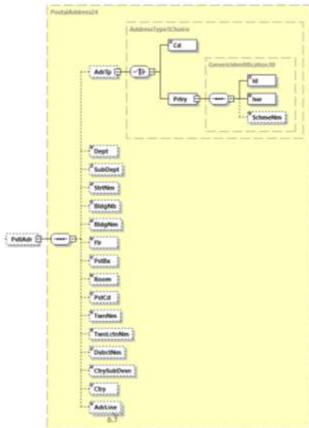
Abbildung 73: pain.002.001.10, Postal Address
