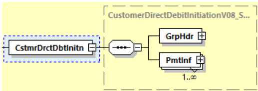
Abbildung 19: pain.008.001.08, Customer Direct Debit Initiation
