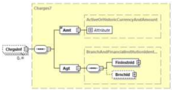
Abbildung 69: pain.002.001.10, Charges Information
