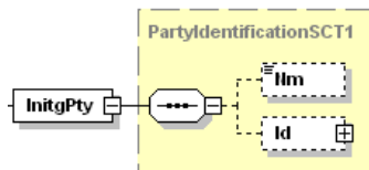
Abbildung 11: pain.001.001.09, Initiating Party
