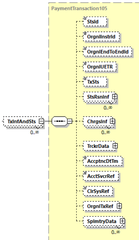
Abbildung 34: pain.002.001.10, Transaction Information and Status
