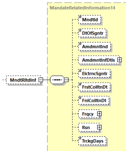
Abbildung 37: pain.002.001.10, Mandate Related Information
