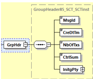
Abbildung 10: pain.001.001.09, Group Header
