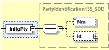
Abbildung 21: pain.008.001.08, Initiating Party
