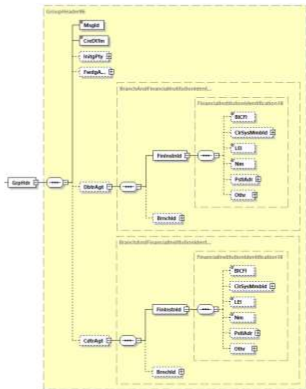
Abbildung 32: pain.002.001.10, Group Header
