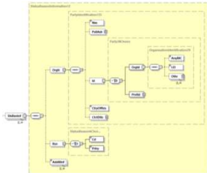
Abbildung 39: pain.002.001.10, Status Reason Information
