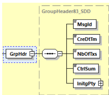
Abbildung 20: pain.008.001.08, Group Header
