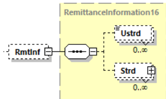
Abbildung 38: pain.002.001.10, Remittance Information
