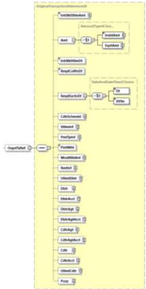
Abbildung 35: pain.002.001.10, Original Transaction Reference
