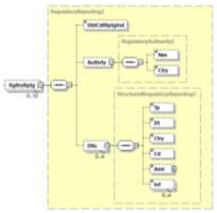
Abbildung 58: pain.001.001.09, Regulatory Reporting
