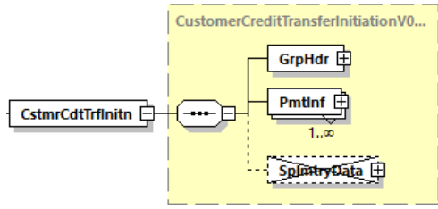
Abbildung 51: pain.001.001.09: Customer Credit Transfer Initiation
