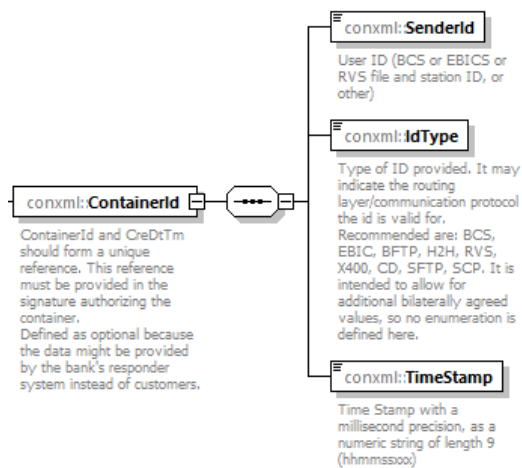
Abbildung 114: container.nnn.001.GBIC4, Container Id
