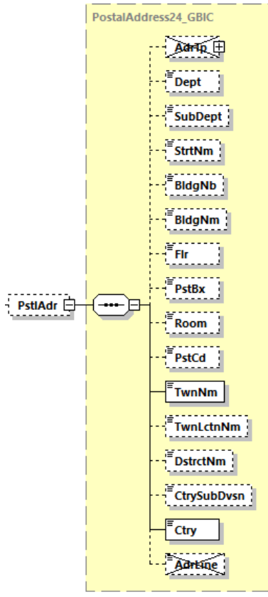
Abbildung 55: pain.001.001.09, Postal Address
