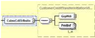
Abbildung 9 pain.001.001.09: Customer Credit Transfer Initiation
