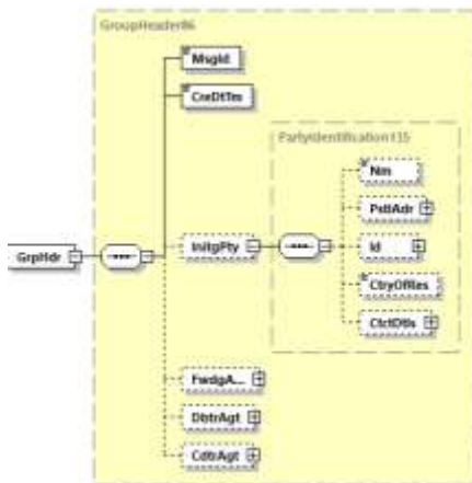
Abbildung 65: pain.002.001.10, Group Header
